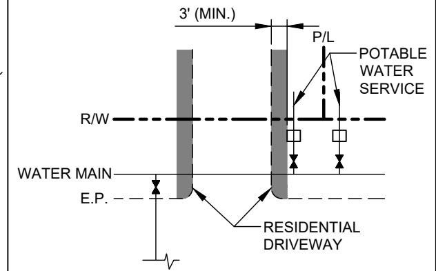
PLAN VIEW (HORIZONTAL SEPARATION)
