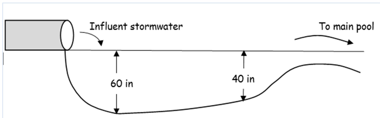
Figure 5: Forebay Diagram
