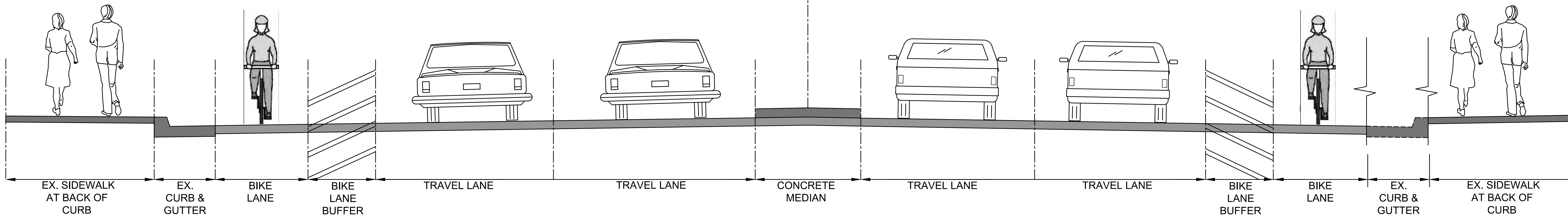
TYPICAL SECTION#2 PARKWOOD AVE. BUFFERED BIKE LANE FROM HAWTHORNE LN TO 1513 PARKWOOD AVE
