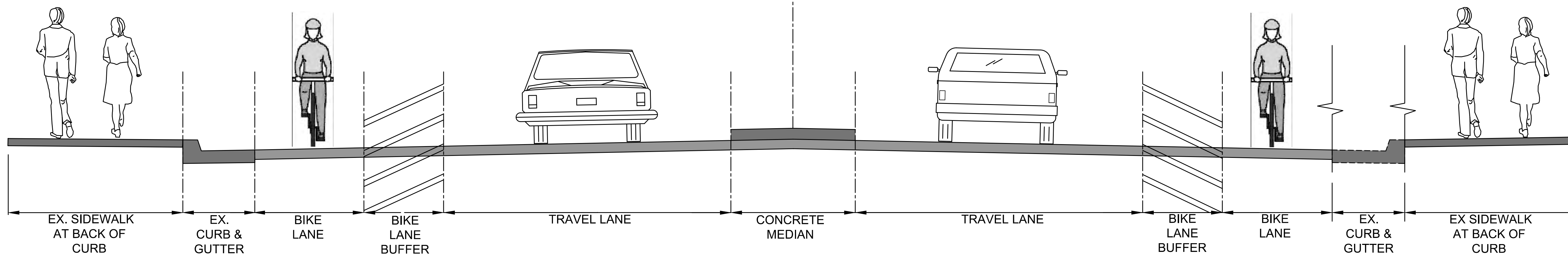
TYPICAL SECTION#1 PARKWOOD AVE. BUFFERED BIKE LANE FROM N. DAVIDSON ST. TO UMSTEAD ST
