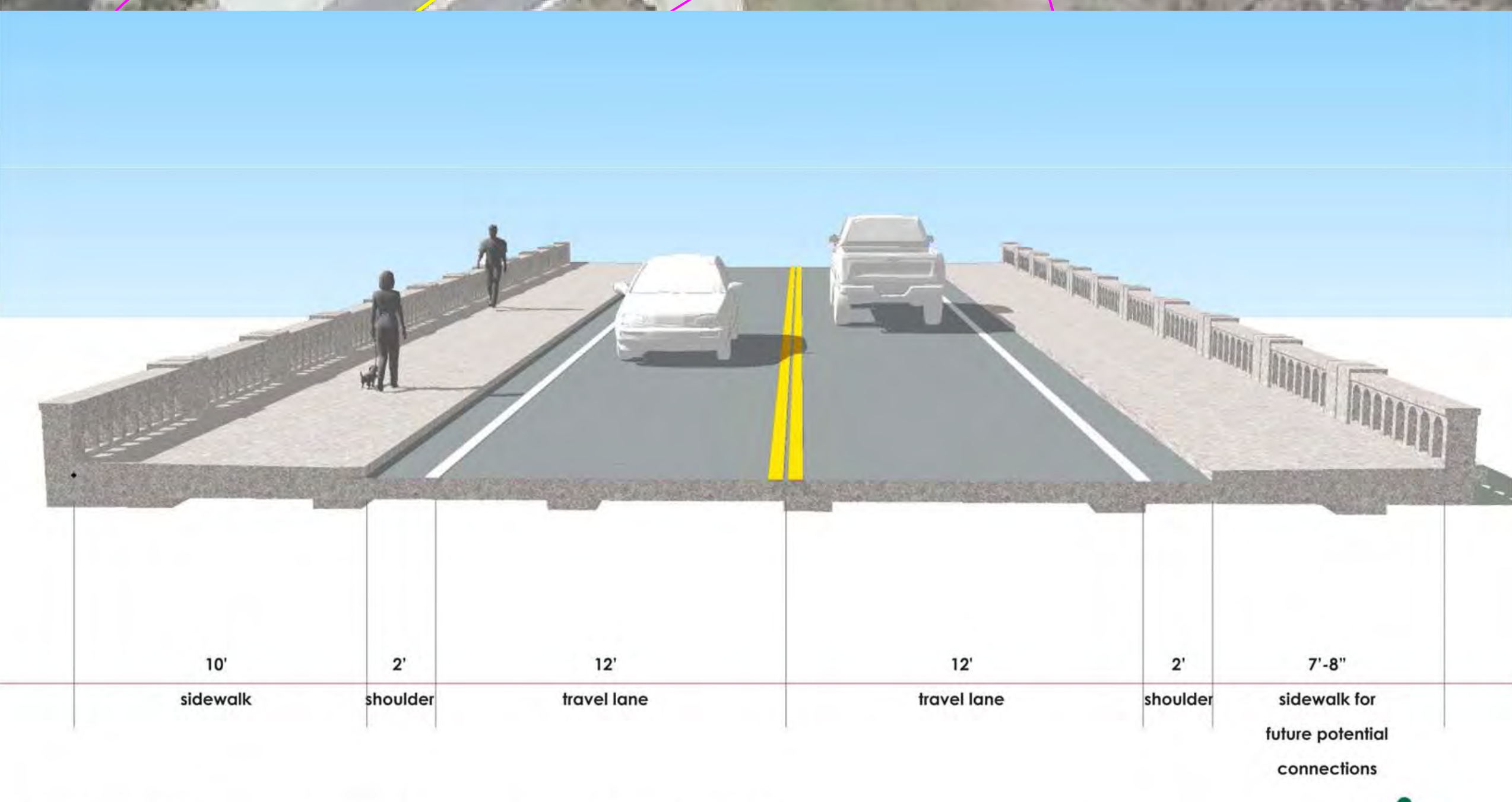
Typical Cross Section (looking East)
